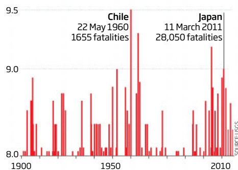
Earthquakes measuring magnitude 8 and above since 1900
