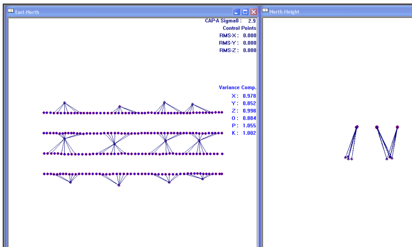
Geometry of Intersecting Rays (Top & Side Views)
