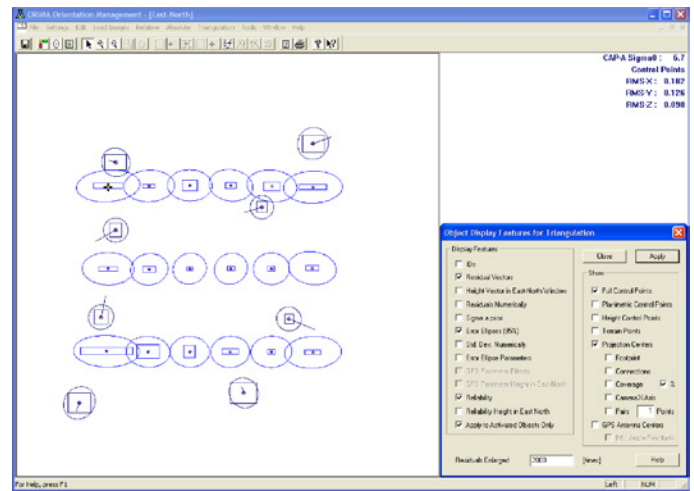
Ground view to analyze quality of block adjustment
