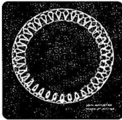
FA - 639 Hz - Antinodes: 38
