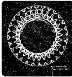
RE - 417 Hz - Antinodes: 28
